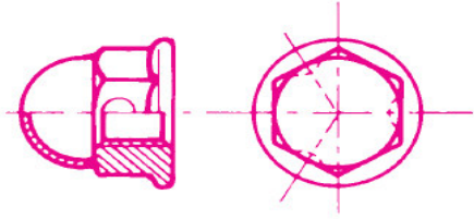
Self-locking flange blind nut
