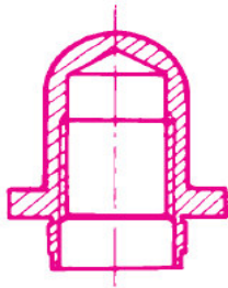
Self-clinching blind nut
