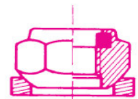
Self-locking conical nut
