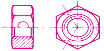
self-locking hexagon nut (din 980)
