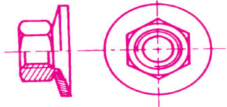
Hex nut with captive spring washer
